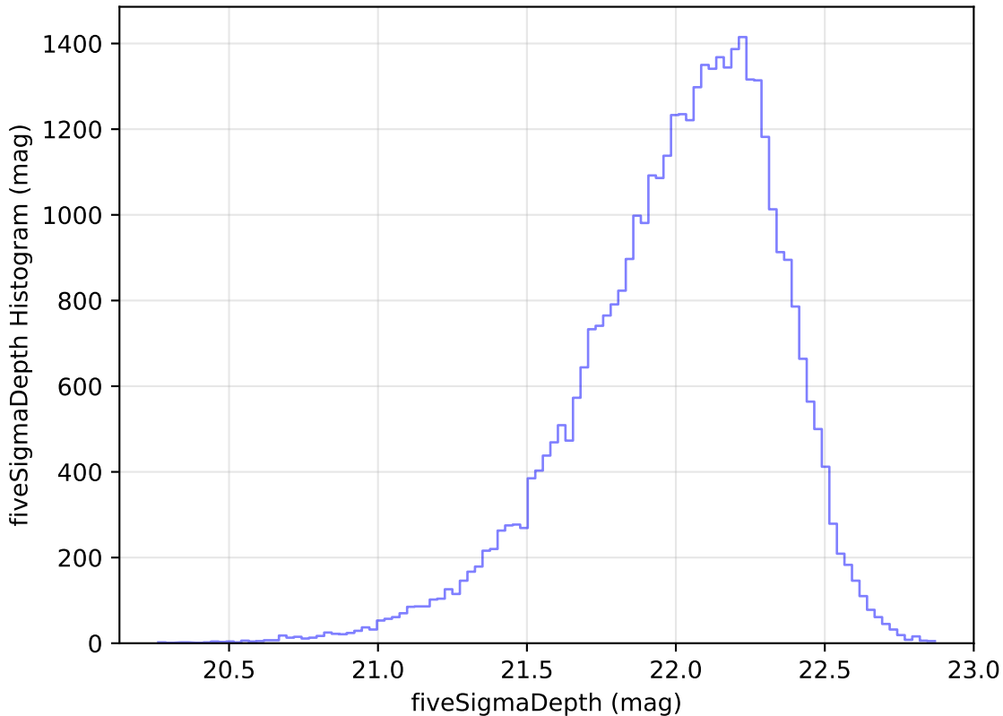
weather_cloudso8v3.4_10yrs Yr 1 y band: fiveSigmaDepth Histogram
