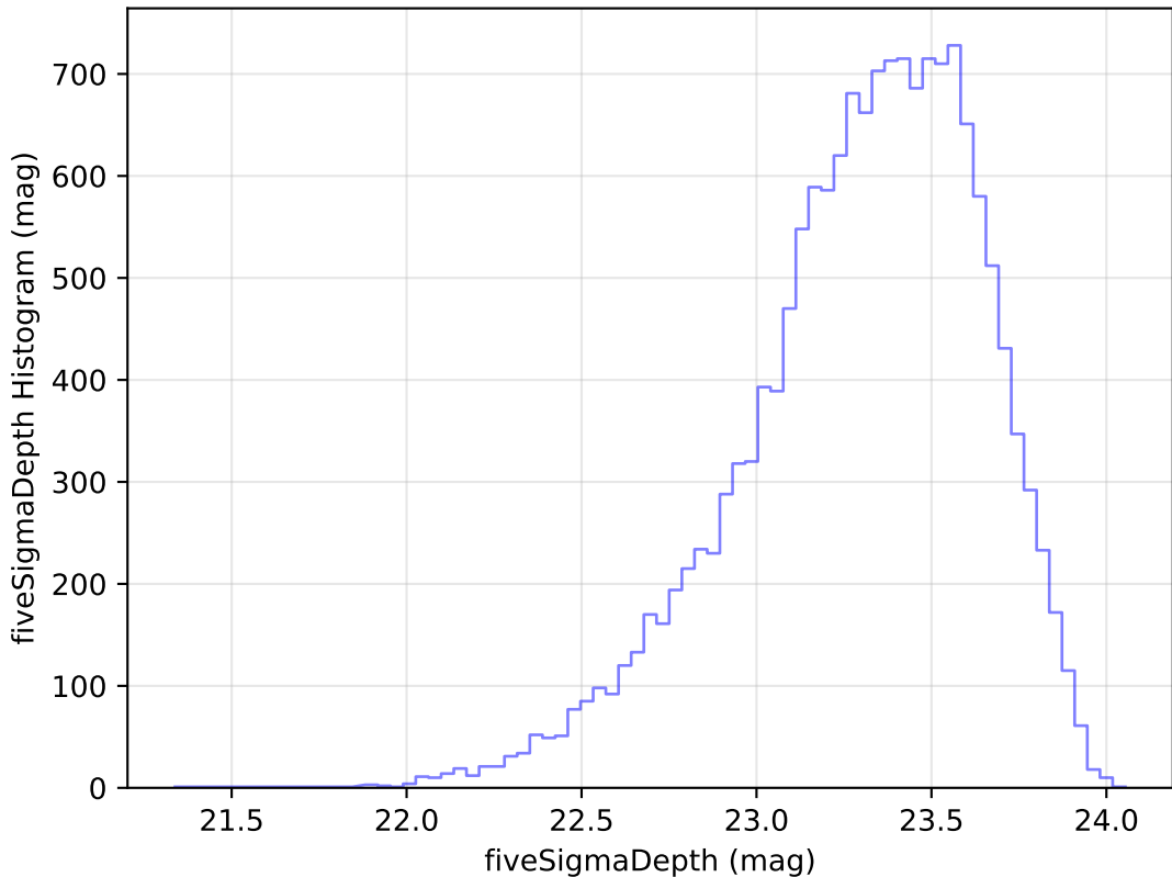
weather_cloudso8v3.4_10yrs Yr 1 u band: fiveSigmaDepth Histogram
