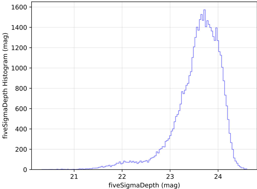
weather_cloudso8v3.4_10yrs Yr 1 i band: fiveSigmaDepth Histogram
