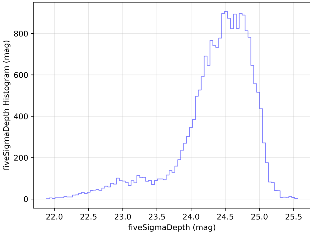
weather_cloudso8v3.4_10yrs Yr 1 g band: fiveSigmaDepth Histogram
