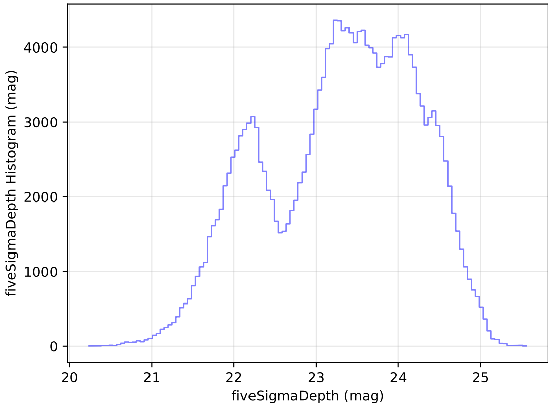
weather_cloudso8v3.4_10yrs Yr 1 all bands: fiveSigmaDepth Histogram
