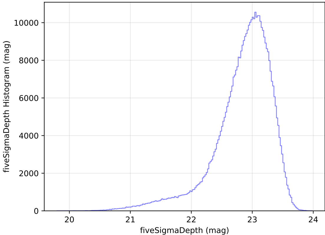
weather_cloudso8v3.4_10yrs WFD z band: fiveSigmaDepth Histogram
