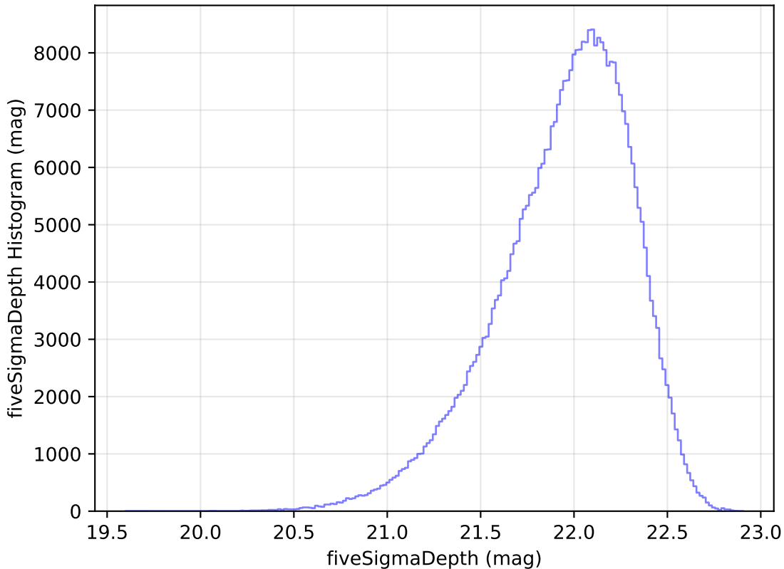
weather_cloudso8v3.4_10yrs WFD y band: fiveSigmaDepth Histogram
