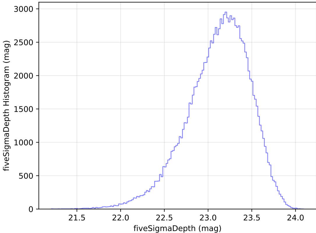
weather_cloudso8v3.4_10yrs WFD u band: fiveSigmaDepth Histogram
