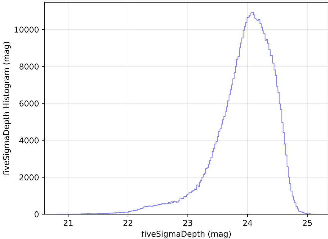
weather_cloudso8v3.4_10yrs WFD r band: fiveSigmaDepth Histogram
