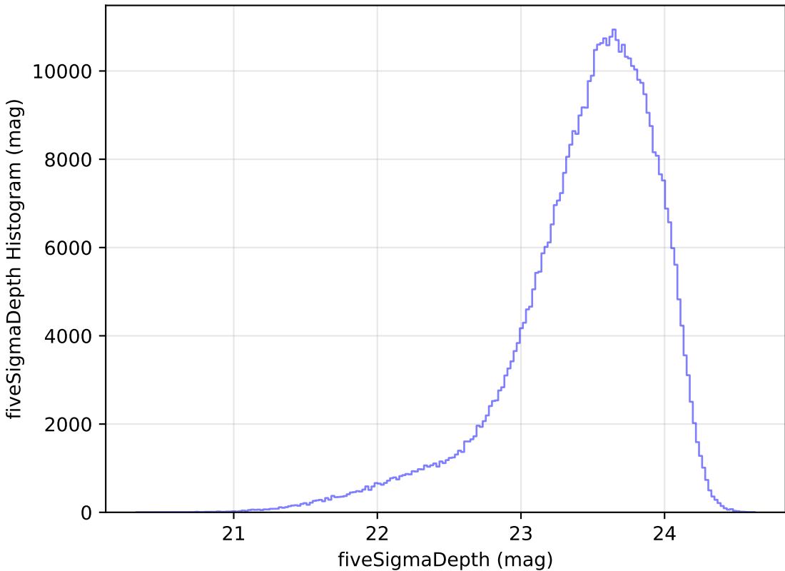
weather_cloudso8v3.4_10yrs WFD i band: fiveSigmaDepth Histogram
