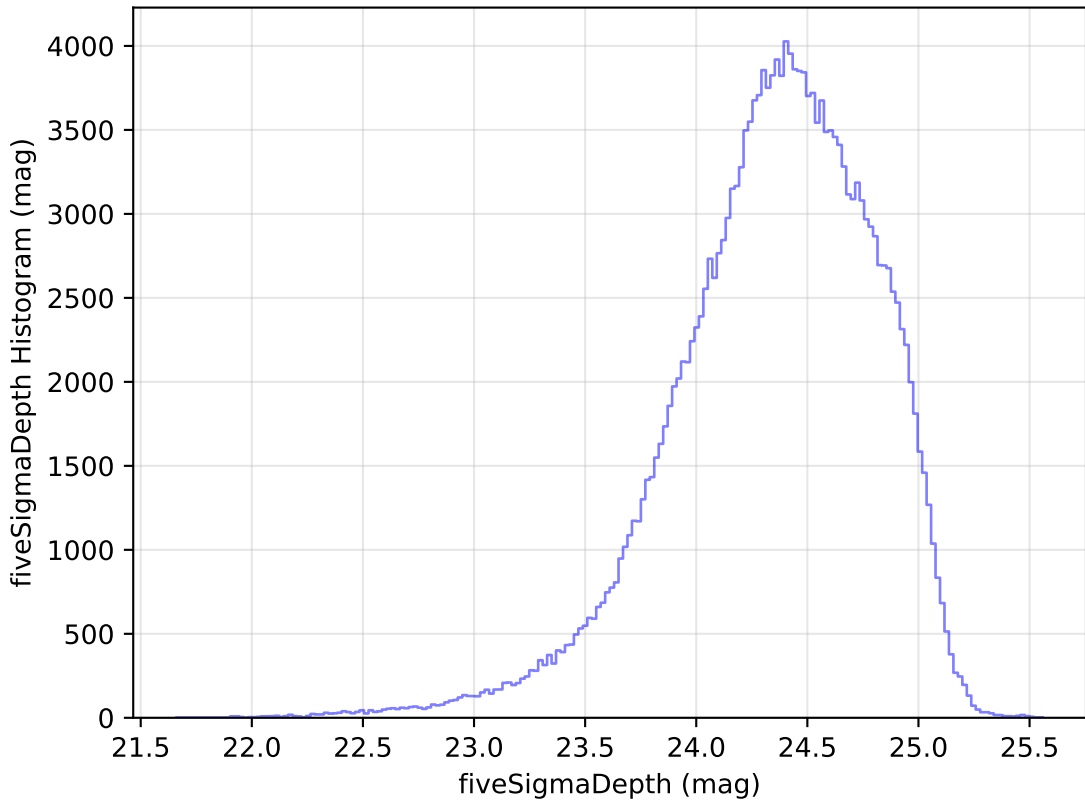
weather_cloudso8v3.4_10yrs WFD g band: fiveSigmaDepth Histogram
