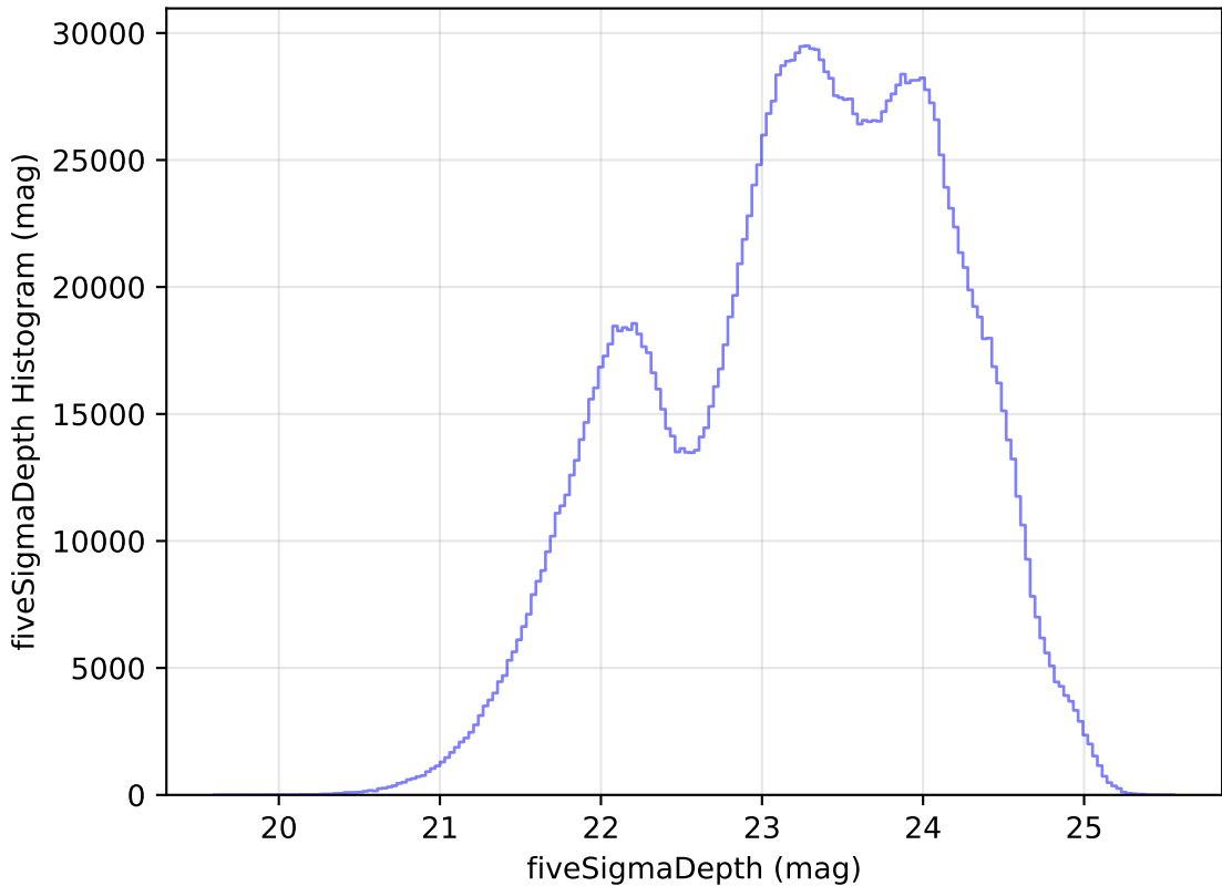
weather_cloudso8v3.4_10yrs WFD all bands: fiveSigmaDepth Histogram
