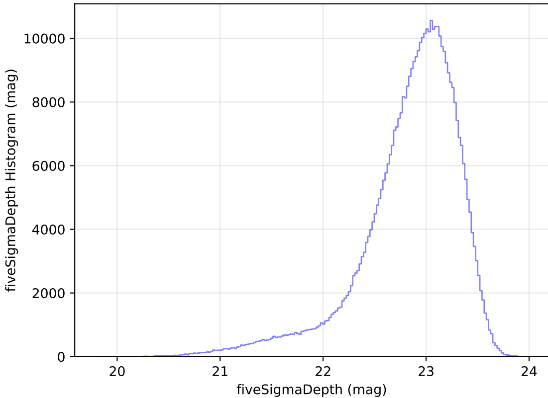
weather_cloudso8v3.4_10yrs All sky z band: fiveSigmaDepth Histogram
