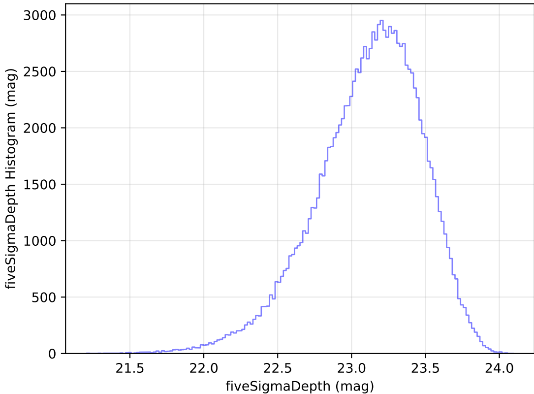
weather_cloudso8v3.4_10yrs All sky u band: fiveSigmaDepth Histogram
