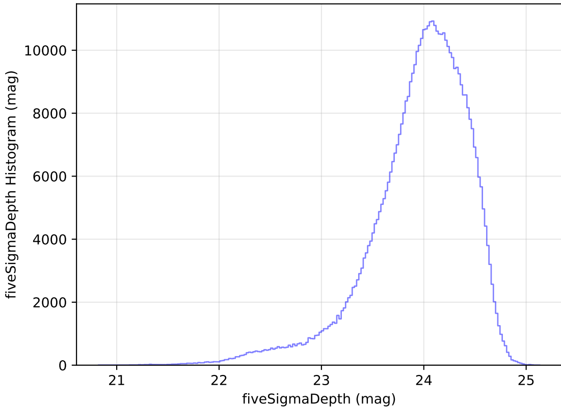
weather_cloudso8v3.4_10yrs All sky r band: fiveSigmaDepth Histogram
