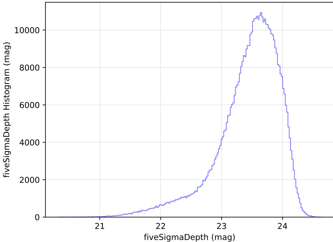
weather_cloudso8v3.4_10yrs All sky i band: fiveSigmaDepth Histogram
