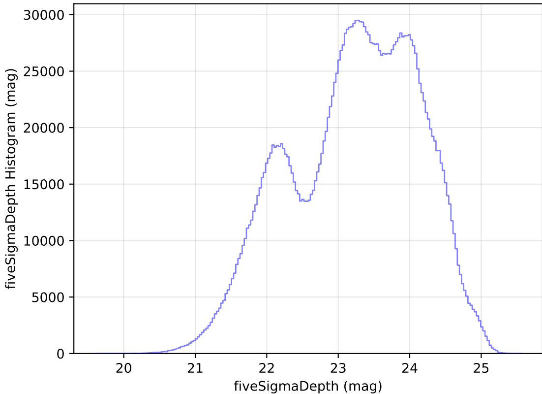
weather_cloudso8v3.4_10yrs All sky all bands: fiveSigmaDepth Histogram
