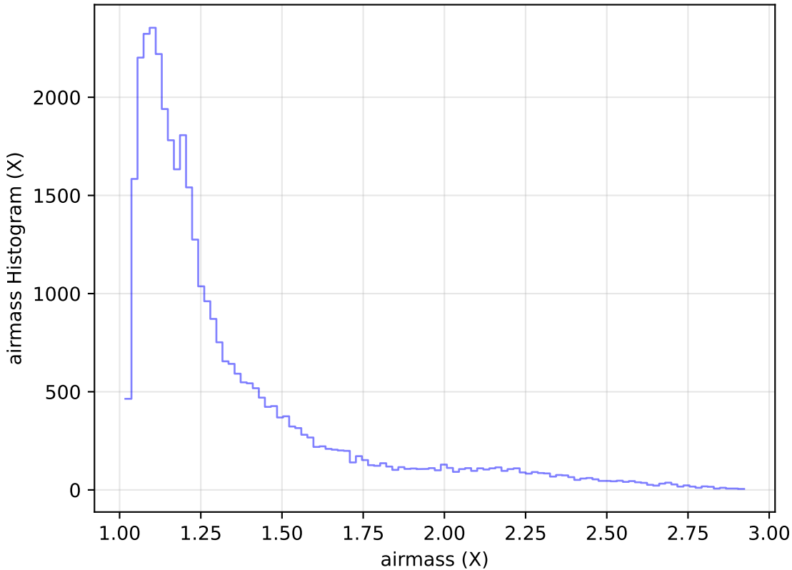
weather_cloudso8v3.4_10yrs Yr 1 z band: airmass Histogram
