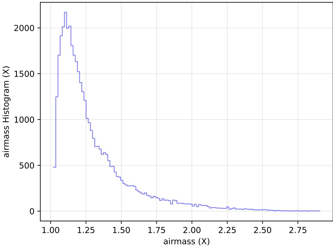
weather_cloudso8v3.4_10yrs Yr 1 y band: airmass Histogram
