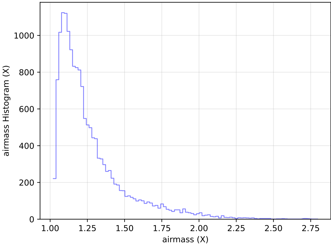
weather_cloudso8v3.4_10yrs Yr 1 u band: airmass Histogram
