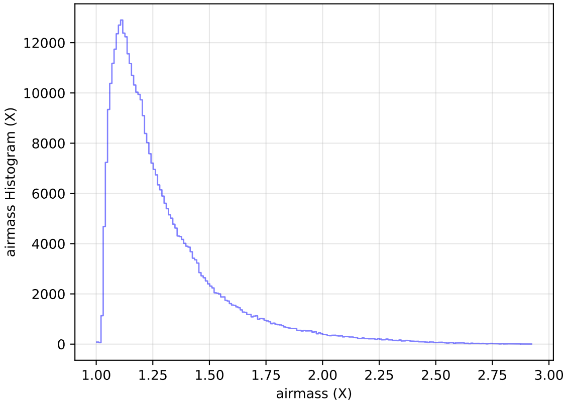
weather_cloudso8v3.4_10yrs WFD y band: airmass Histogram
