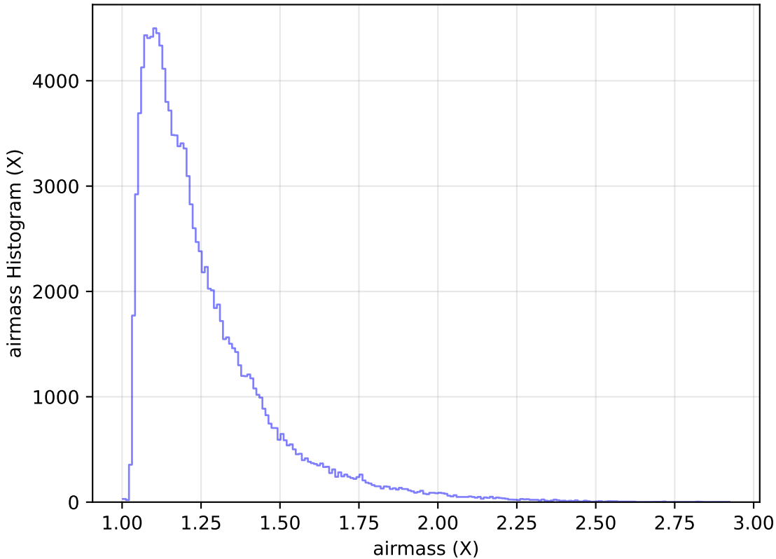
weather_cloudso8v3.4_10yrs WFD u band: airmass Histogram
