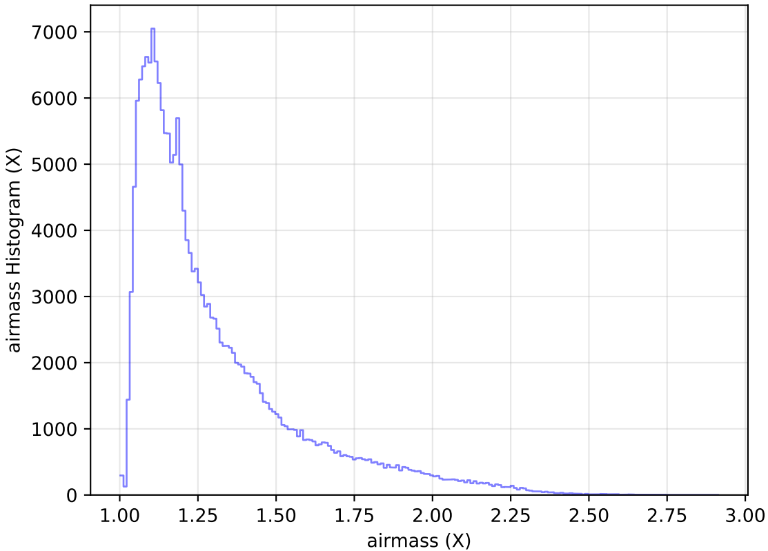
weather_cloudso8v3.4_10yrs WFD g band: airmass Histogram
