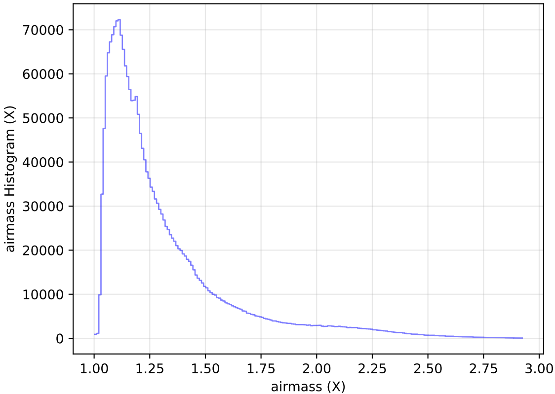
weather_cloudso8v3.4_10yrs WFD all bands: airmass Histogram
