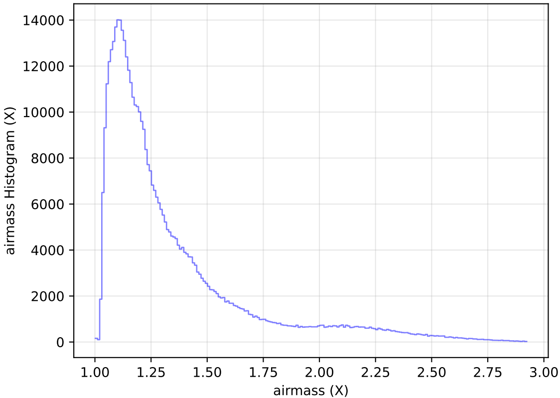
weather_cloudso8v3.4_10yrs All sky z band: airmass Histogram
