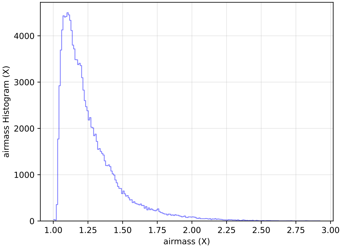
weather_cloudso8v3.4_10yrs All sky u band: airmass Histogram
