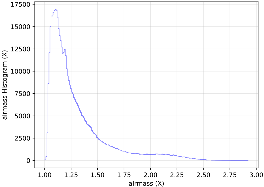
weather_cloudso8v3.4_10yrs All sky r band: airmass Histogram
