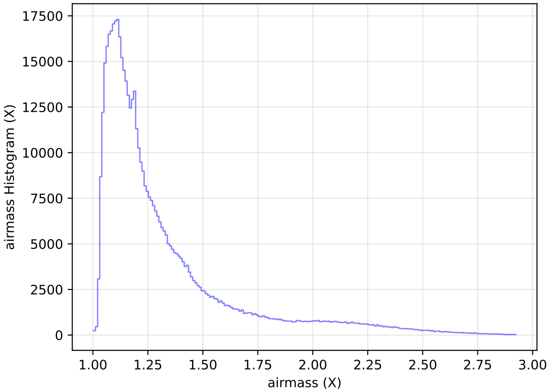
weather_cloudso8v3.4_10yrs All sky i band: airmass Histogram
