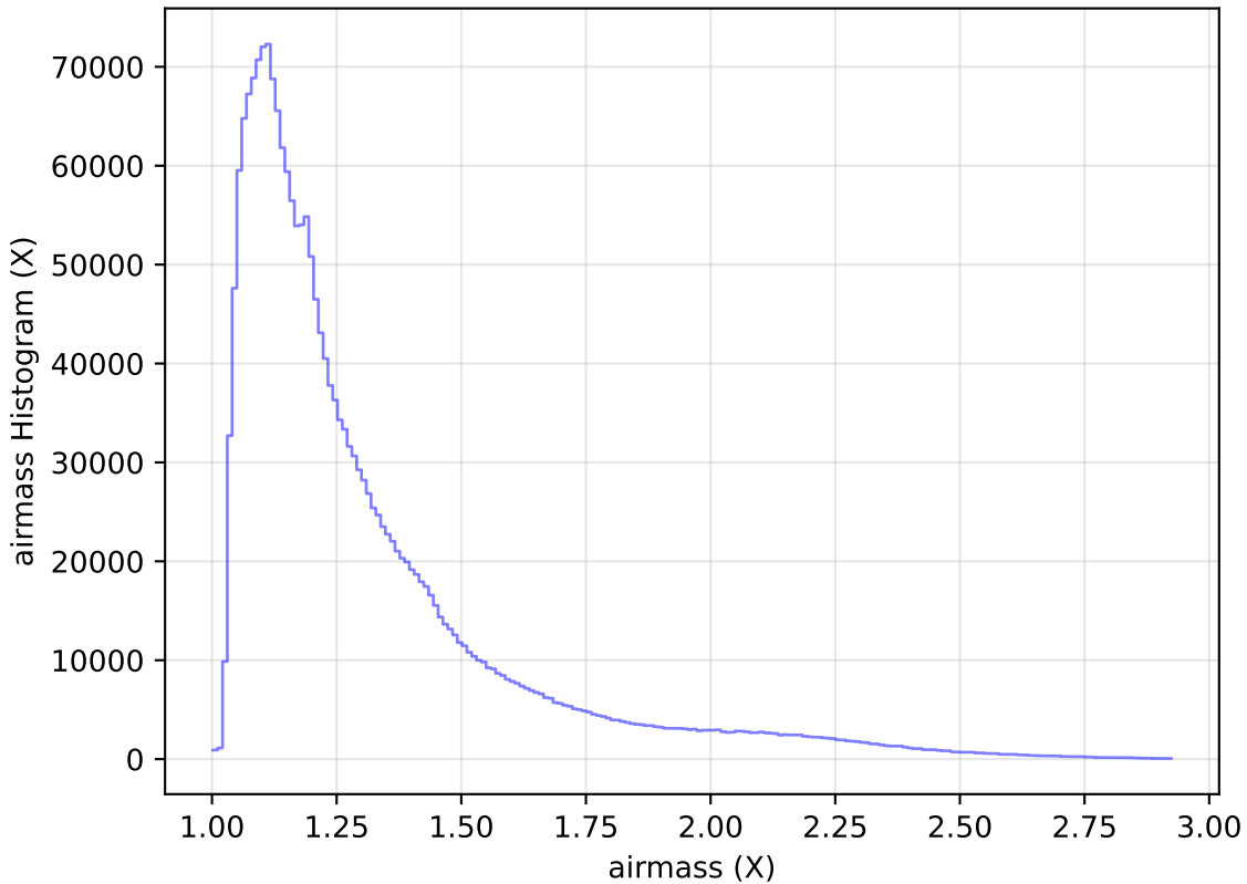
weather_cloudso8v3.4_10yrs All sky all bands: airmass Histogram
