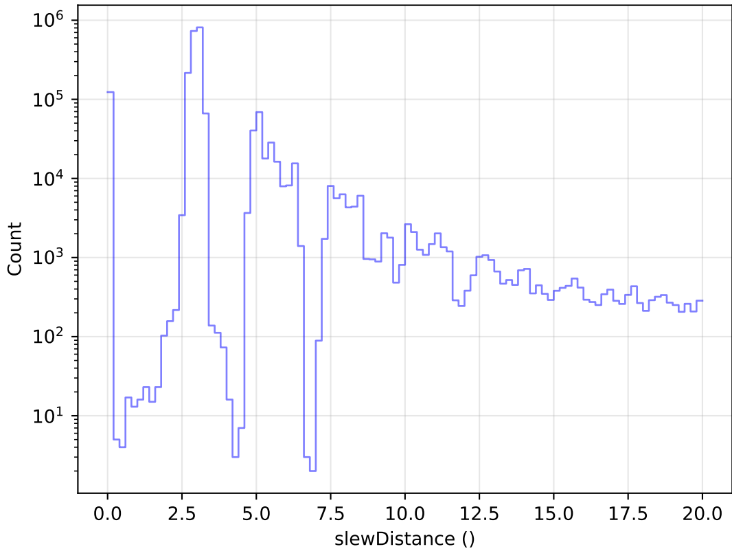
weather_cloudso8v3.4_10yrs All visits: Zoom Slew Distance Histogram
