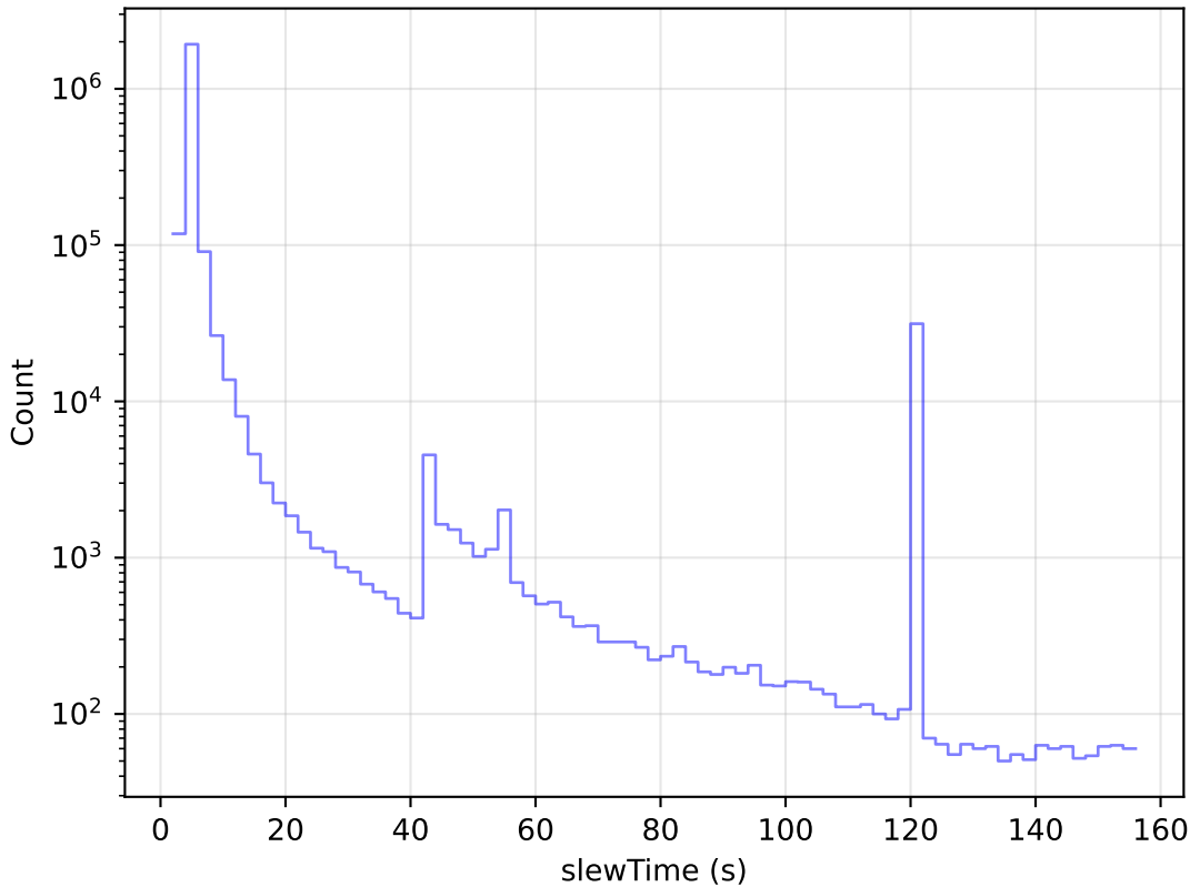
weather_cloudso8v3.4_10yrs All visits: Slew Time Histogram
