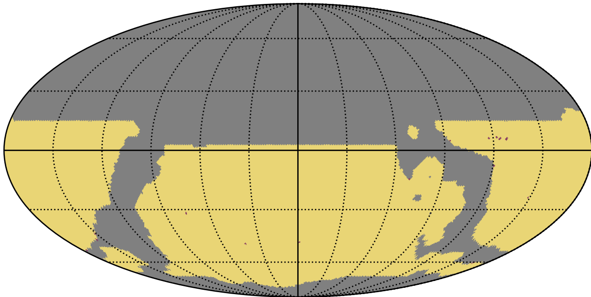
weather_cloudso8v3.4_10yrs WFD: RapidRevisits
