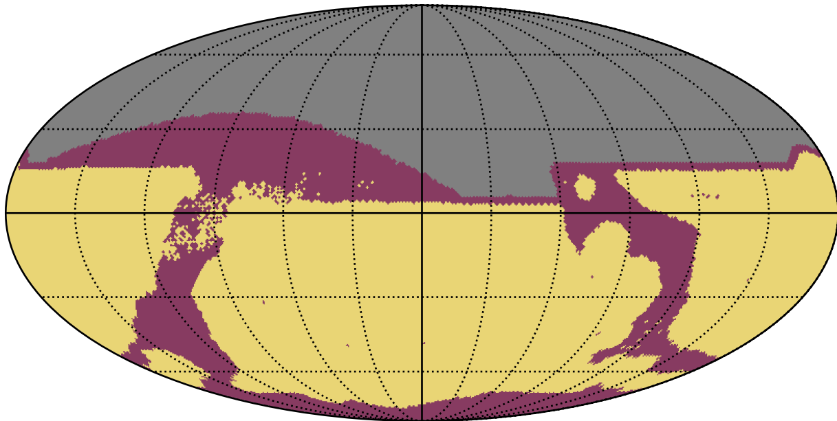
weather_cloudso8v3.4_10yrs All sky: RapidRevisits
