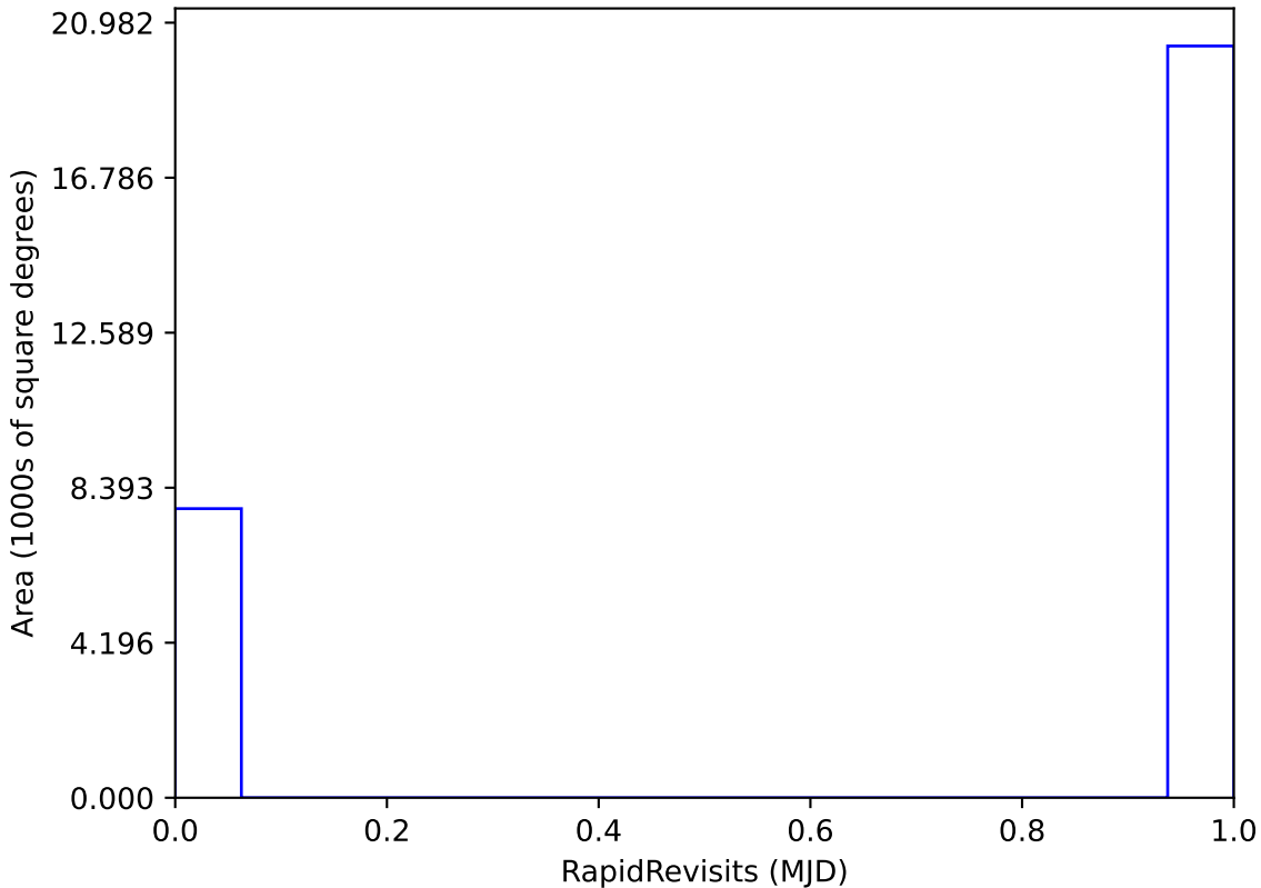
weather_cloudso8v3.4_10yrs All sky: RapidRevisits
