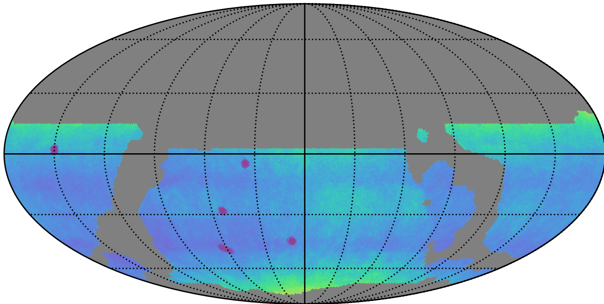
weather_cloudso8v3.4_10yrs WFD: Proper Motion Uncert @ 24.0
