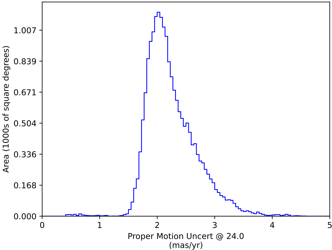
weather_cloudso8v3.4_10yrs WFD: Proper Motion Uncert @ 24.0
