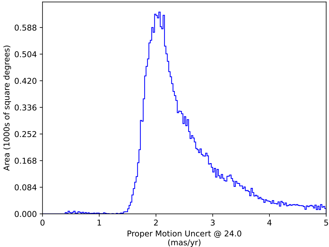
weather_cloudso8v3.4_10yrs All sky: Proper Motion Uncert @ 24.0
