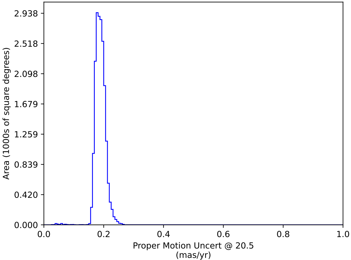
weather_cloudso8v3.4_10yrs WFD: Proper Motion Uncert @ 20.5
