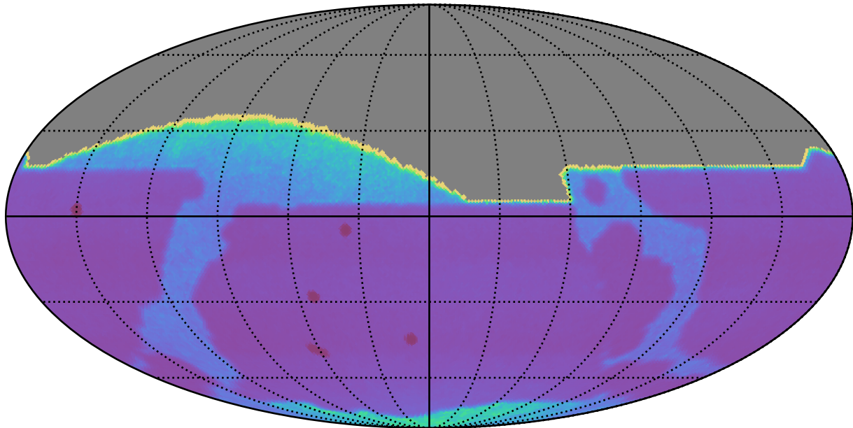
weather_cloudso8v3.4_10yrs All sky: Proper Motion Uncert @ 20.5
