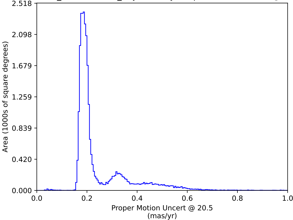
weather_cloudso8v3.4_10yrs All sky: Proper Motion Uncert @ 20.5
