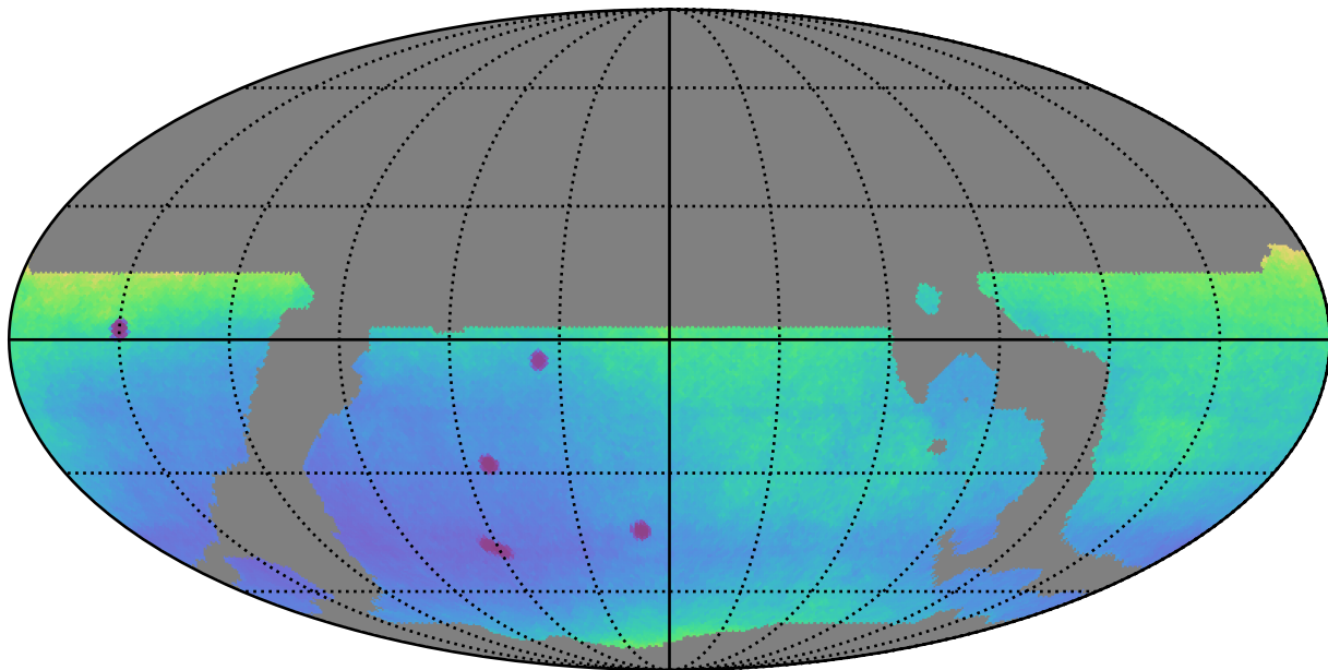
weather_cloudso8v3.4_10yrs WFD: Parallax Uncert @ 24.0
