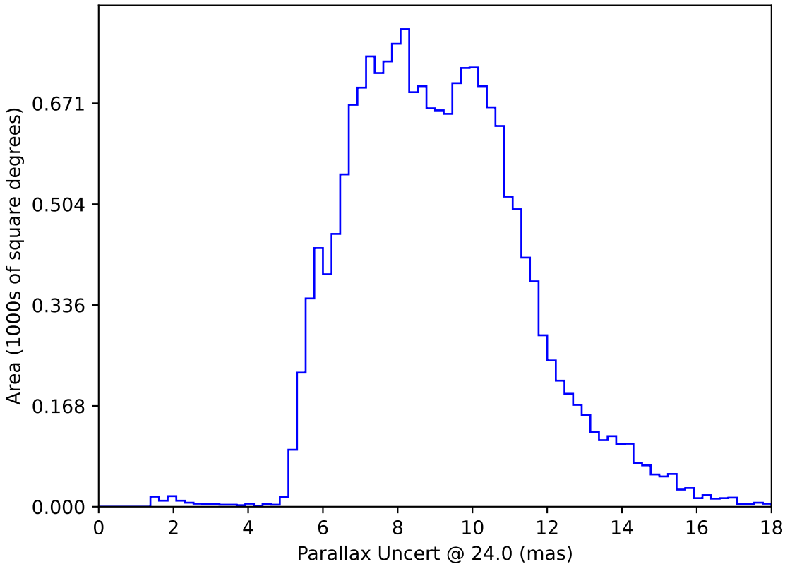
weather_cloudso8v3.4_10yrs WFD: Parallax Uncert @ 24.0
