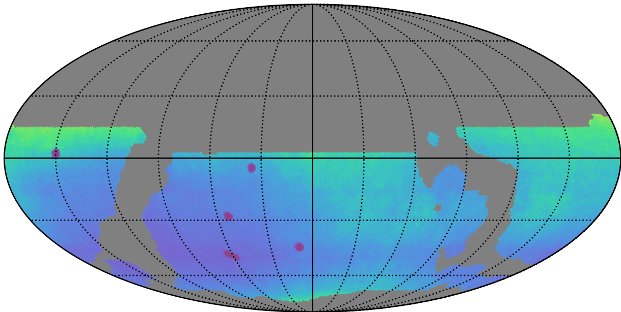
weather_cloudso8v3.4_10yrs WFD: Parallax Uncert @ 22.4
