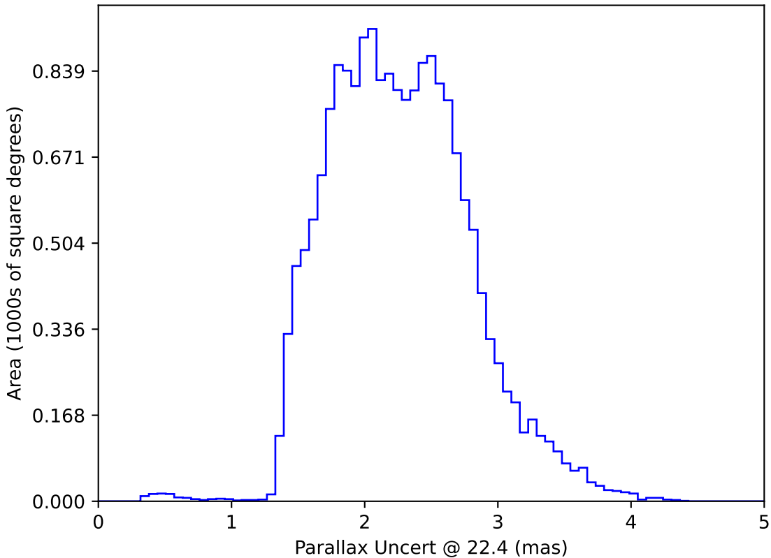
weather_cloudso8v3.4_10yrs WFD: Parallax Uncert @ 22.4
