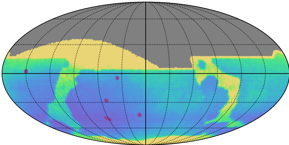
weather_cloudso8v3.4_10yrs All sky: Parallax Uncert @ 22.4
