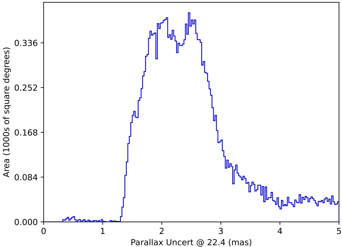
weather_cloudso8v3.4_10yrs All sky: Parallax Uncert @ 22.4
