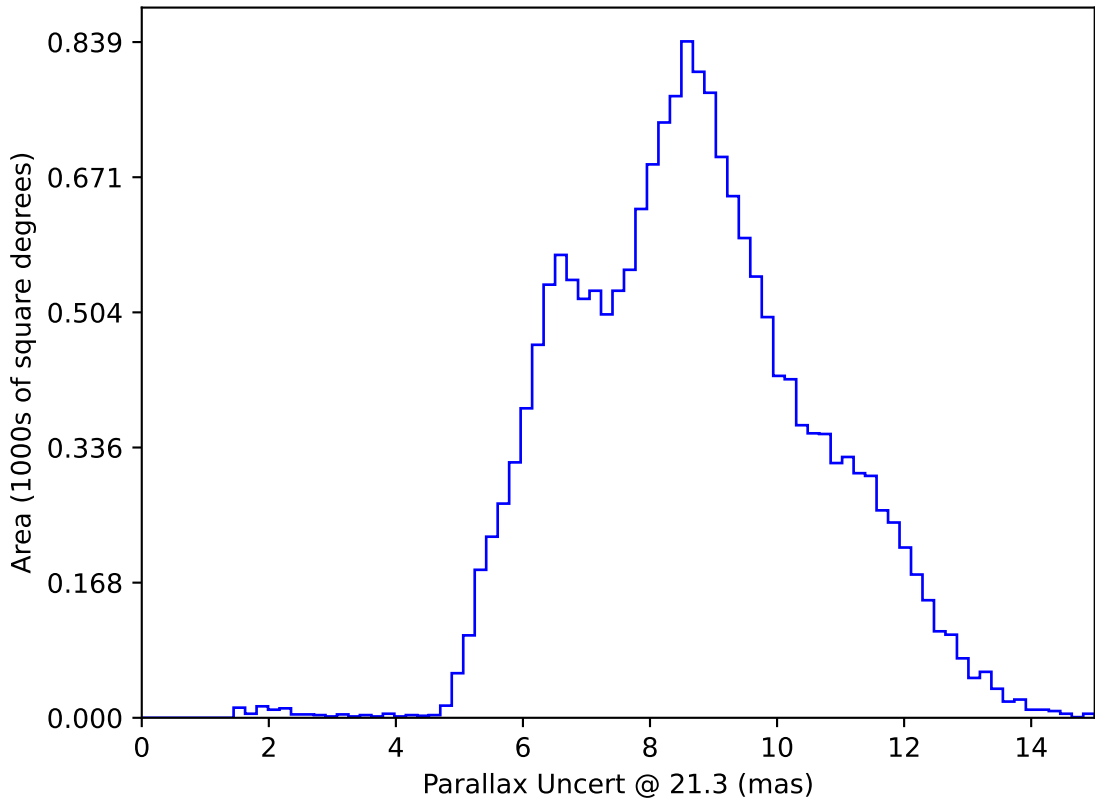
weather_cloudso8v3.4_10yrs WFD y band only: Parallax Uncert @ 21.3
