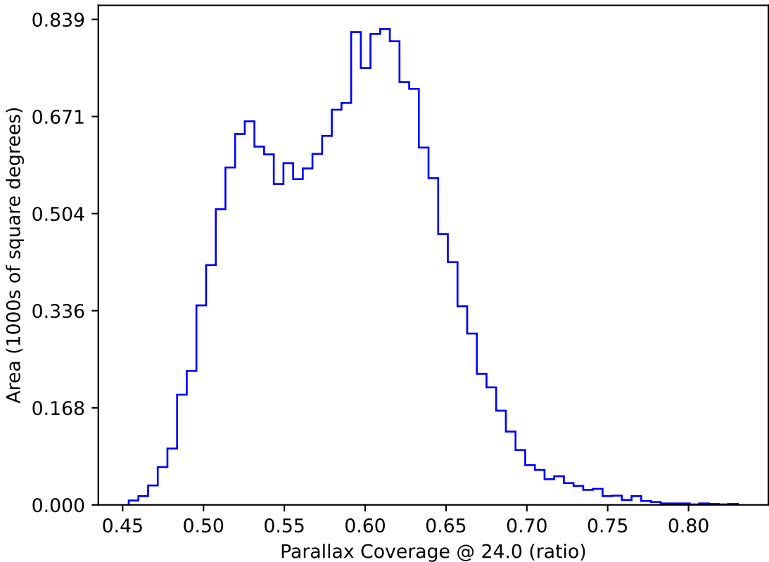
weather_cloudso8v3.4_10yrs WFD: Parallax Coverage @ 24.0
