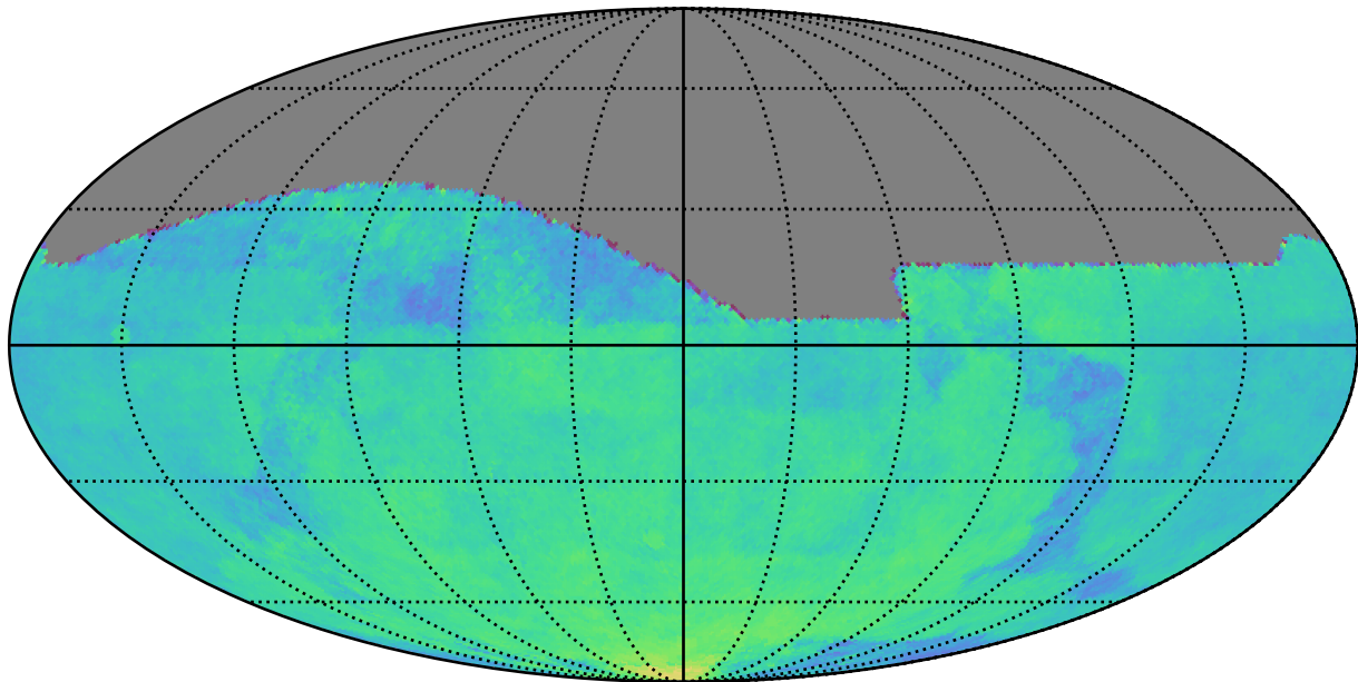
weather_cloudso8v3.4_10yrs All sky: Parallax Coverage @ 24.0
