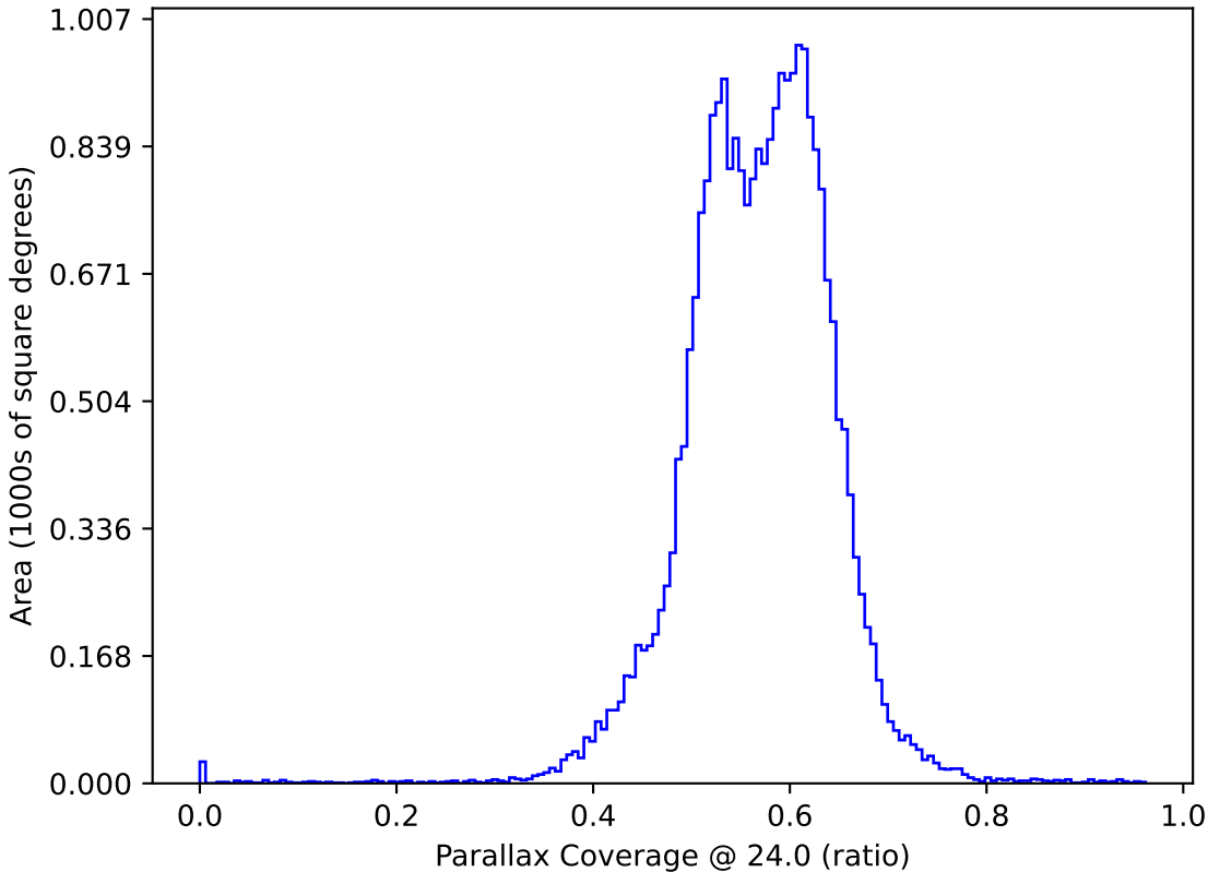
weather_cloudso8v3.4_10yrs All sky: Parallax Coverage @ 24.0
